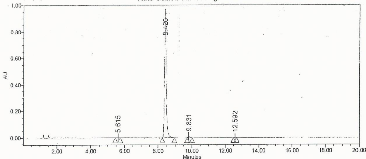
Auto-Scaled Chromatogram
